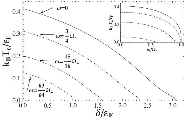
FIG. 2. Main panel: T_c(\delta, \omega) in a spherical trap for a range of rotation rates \omega as a function of \delta . Inset: T_c(\delta, \omega) for a range of detuning \delta = \{0, 0.9, 1.8, 2.7\}\epsilon_F as a function of \omega with the top line being for \delta = 0 . In both cases, N = 10^7 and \gamma = 1/3 .
